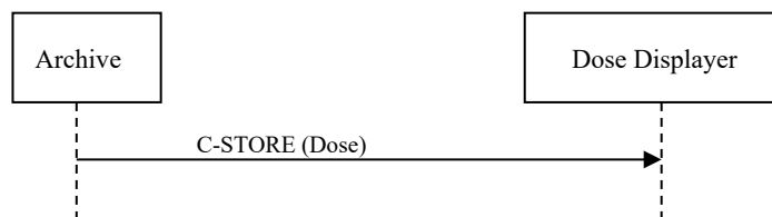
Figure 3.11.4-1: Interaction Diagram
