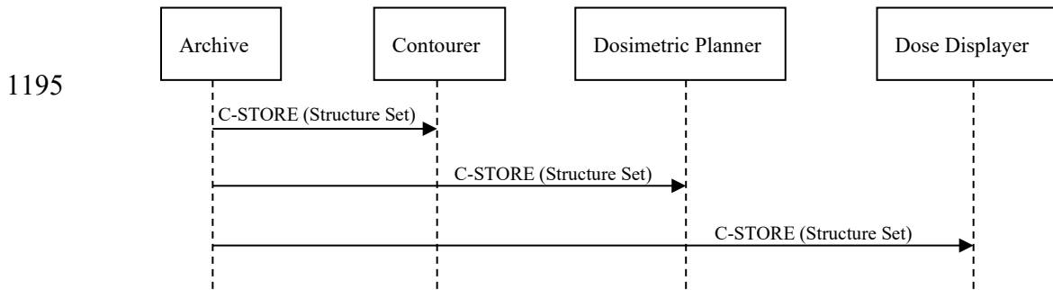
Figure 3.8.4-1: Interaction Diagram
