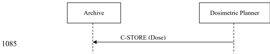
Figure 3.6.4-1: Interaction Diagram
