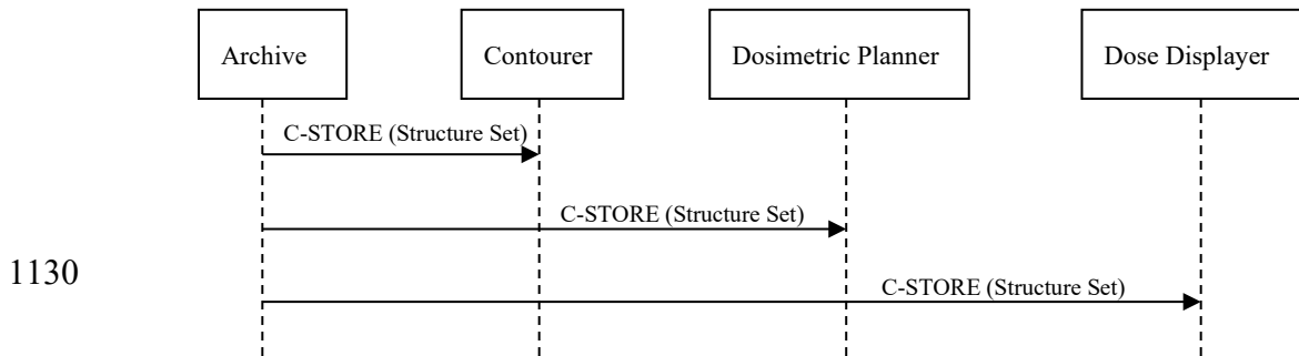
Figure 3.7.4-1: Interaction Diagram
