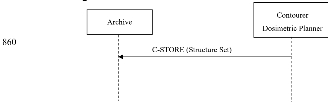
Figure 3.2.4-1: Interaction Diagram
