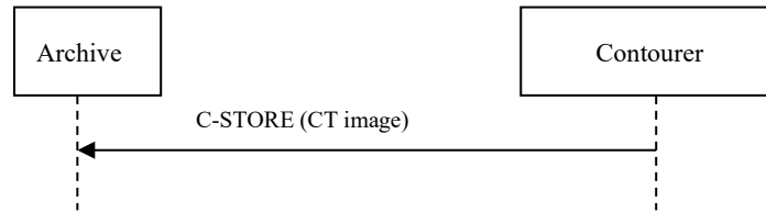
Figure 3.13.4-1: Interaction Diagram
