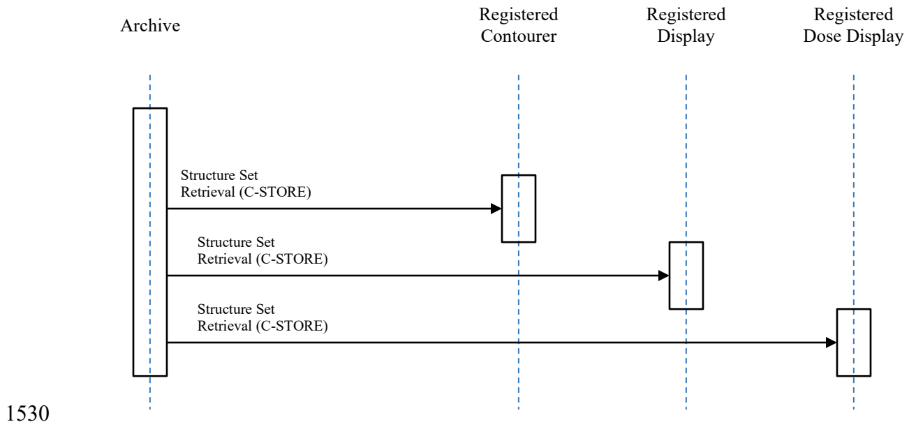
Figure 3.15.4-1: Interaction Diagram
