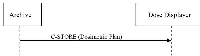
Figure 3.10.4-1: Interaction Diagram
