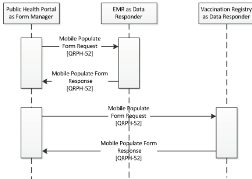
540 Figure X.4.2.2.2-2: Use Case 2 - Public Health Enrollment Form Population Process Flow
