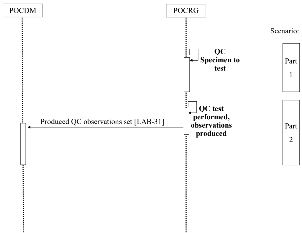
Figure 6.4.2.5.2-1: Process Flow in LPOCT Profile
