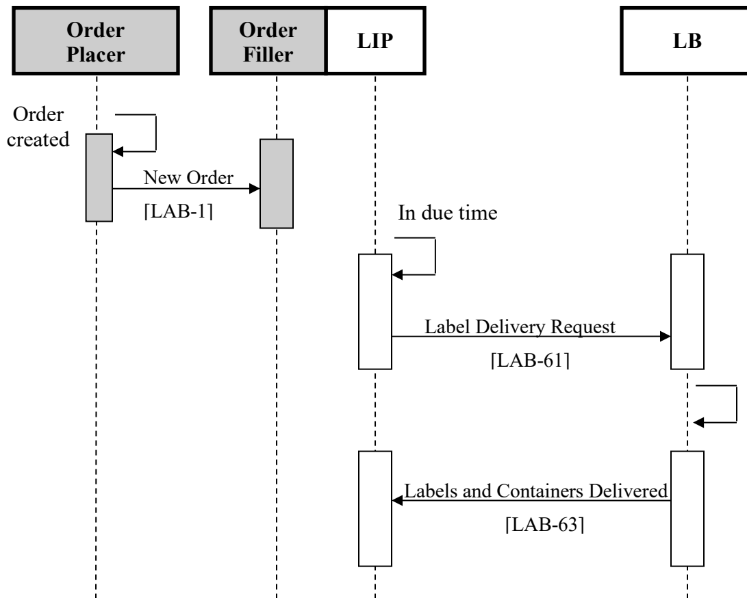
1690 Figure 7.4.2.3.2-1: Filler Requesting Process Flow in LBL Profile
