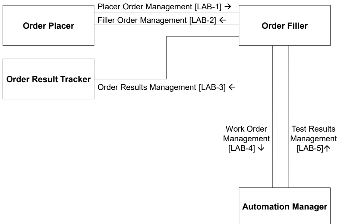
Figure 3.1-1: LTW Actor Diagram
