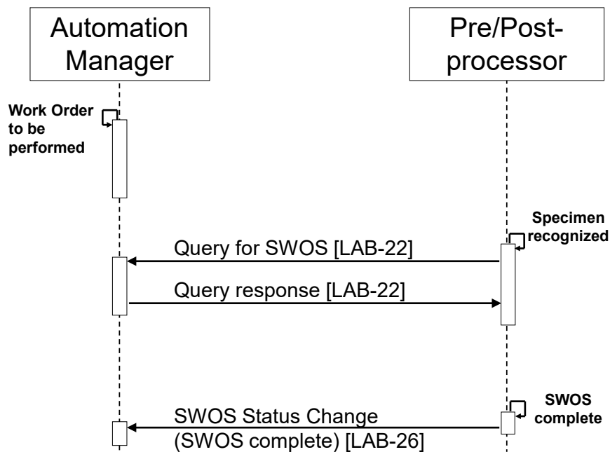
770 Figure 4.4.2.2.2-1: SWOS Queried Process Flow in LDA Profile
