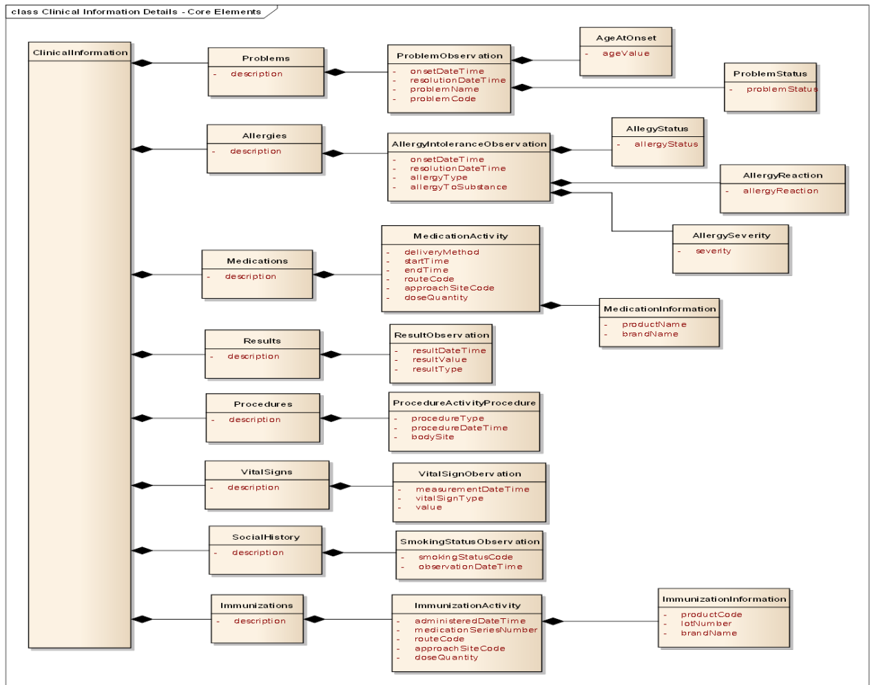
Figure 2.2.3.2-1: Detailed Clinical Data
