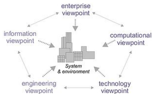
Figure 1.5-1: RM-ODP viewpoints applied to a System and Environment 1
