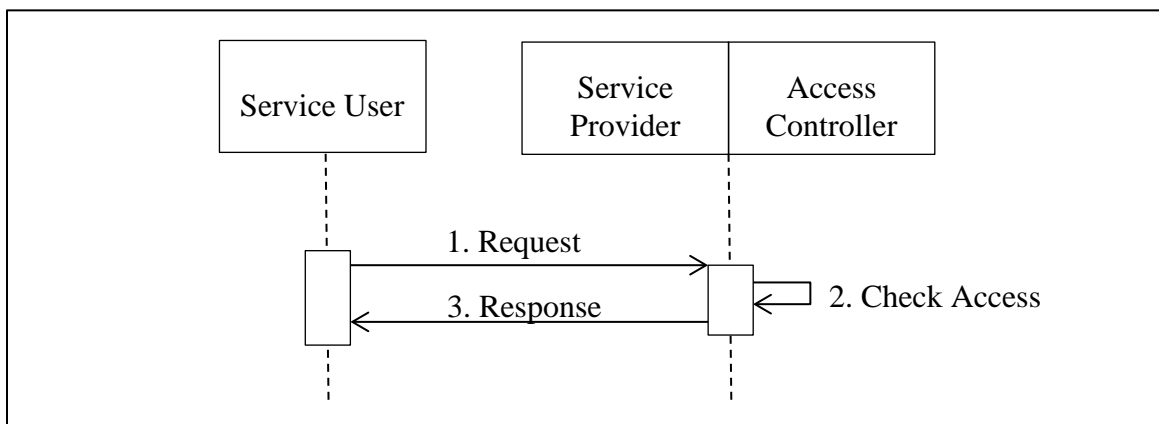
710 Figure 2.3.3.5-1: Access Control
