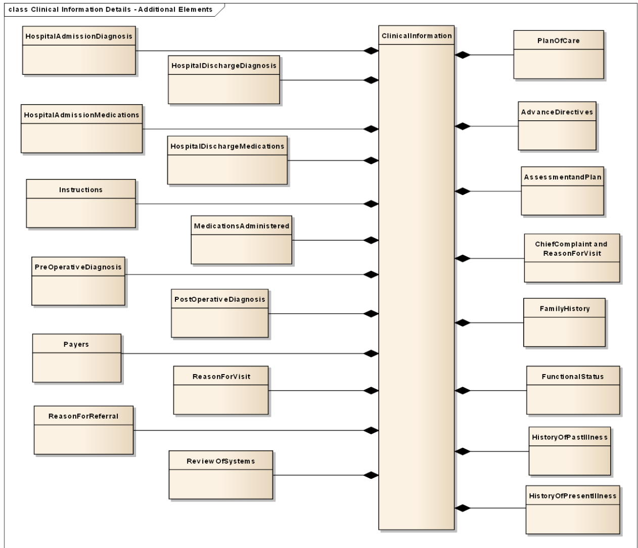
Figure 2.2.3.2-2: More Detailed Clinical Data
