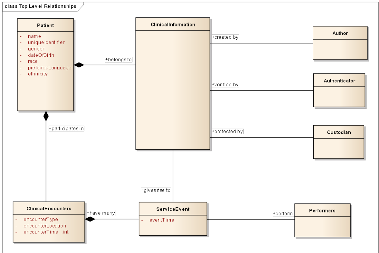
Figure 2.2.3.1-1: Contextual Information Model
