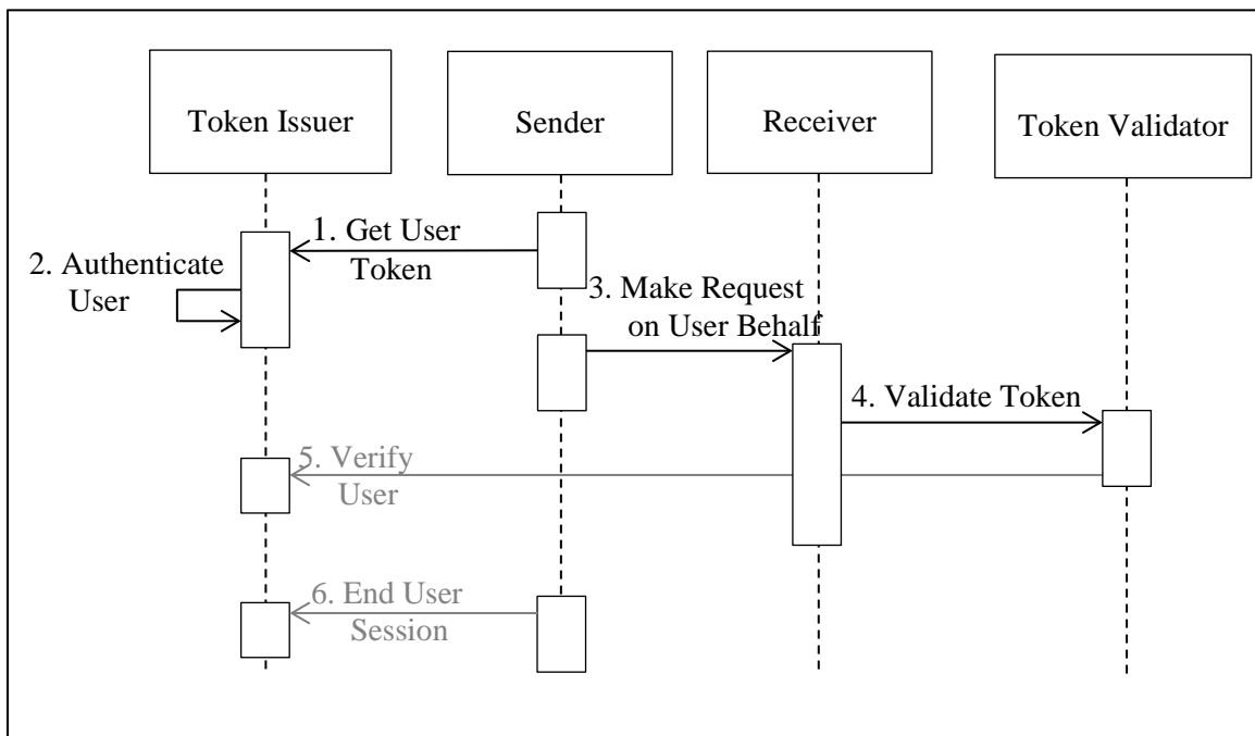
Figure 2.3.3.4-1: User Authentication and/or Authorization
