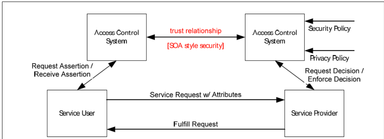
Figure 2.3.3.5-2: Loosely Coupled Access Control Implementation
