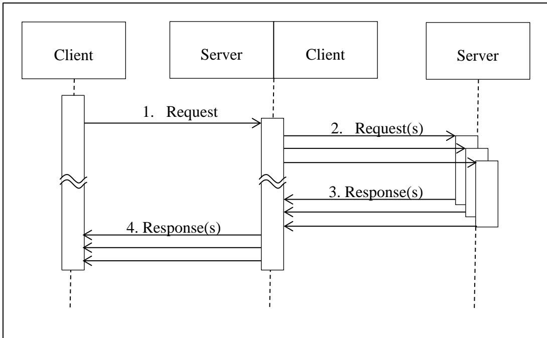
Figure 2.3.2-1: General Federation Pattern
