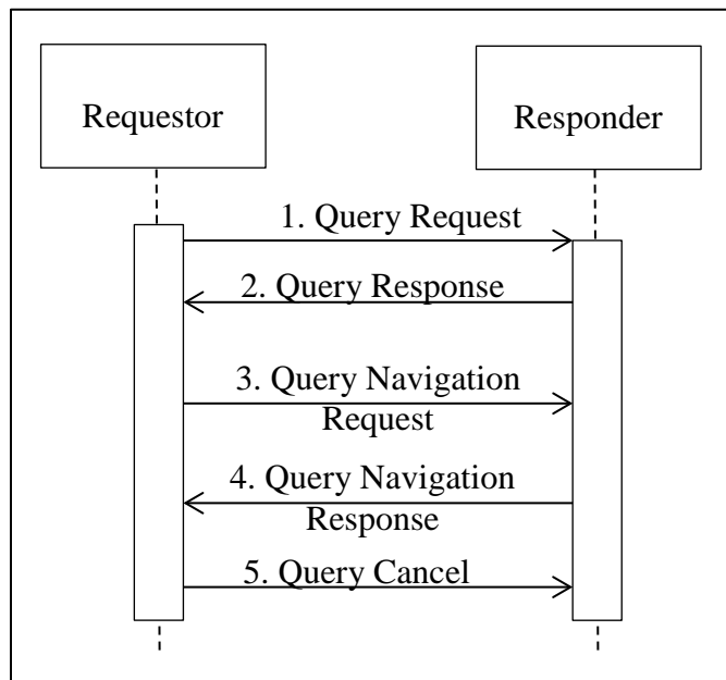
Figure 2.3.1.2-1: Stateful Query Request with Batched Responses
