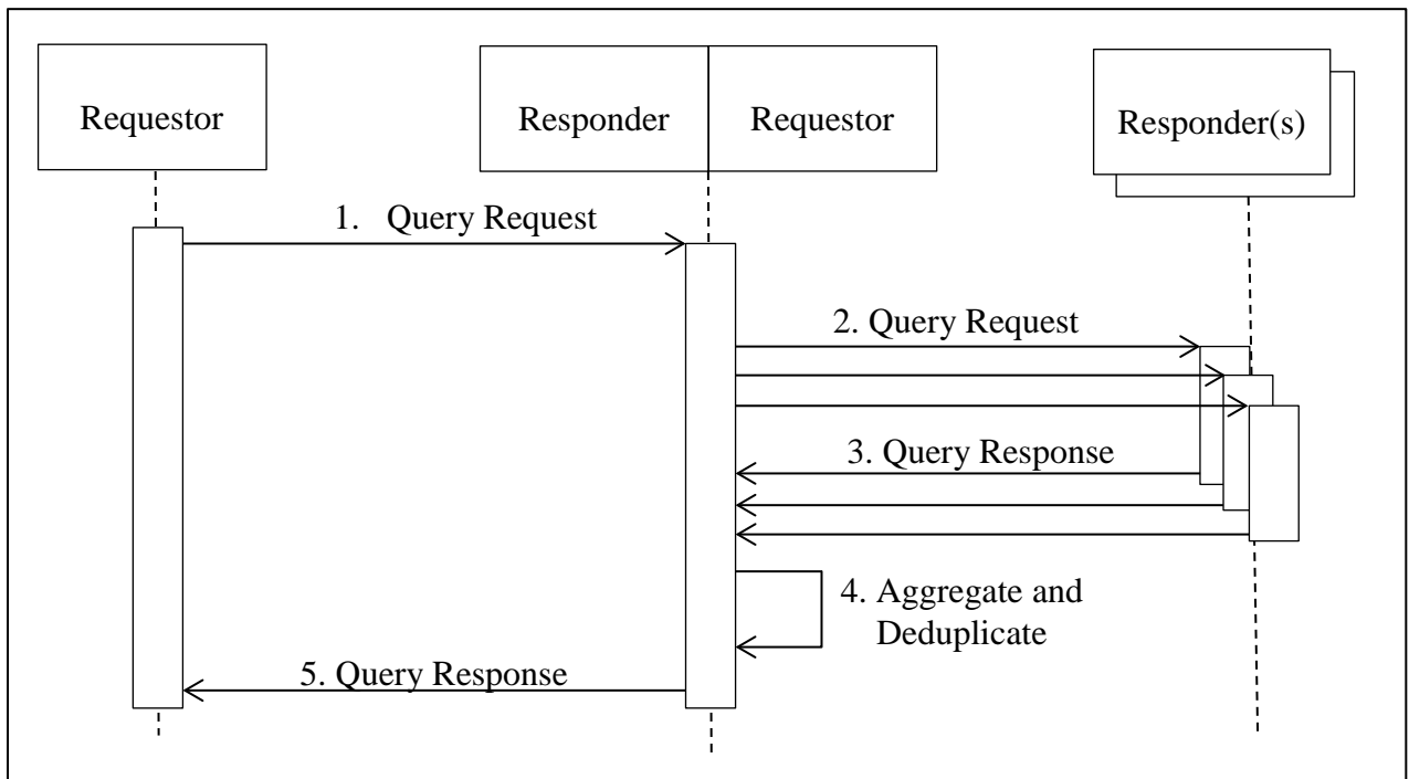
Figure 2.3.2.1-1: Federated Request/Response Pattern
