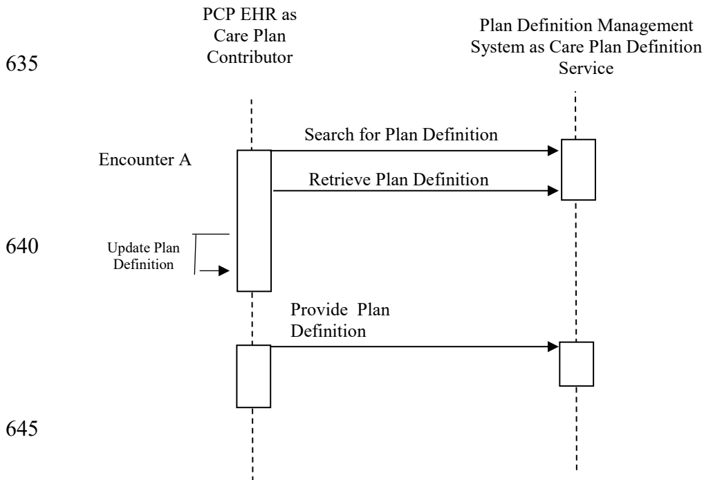
Figure X.4.2.1.1.1-1: Encounter A: Basic Process Flow for Plan Definition
