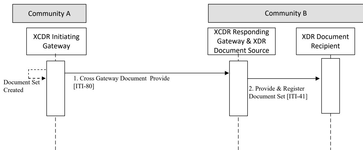
390 Figure 40.4.2.2.2-1: Remote Community with XDR Process Diagram
