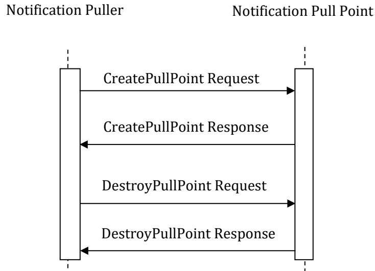
Figure 3.69.4-1: Interaction Diagram
