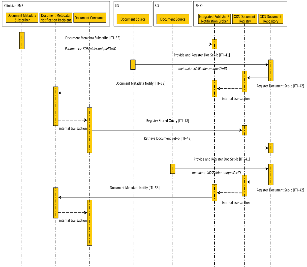
Figure 26.4.2.6.2-1: Interaction Diagram for Folder subscription Use Case
