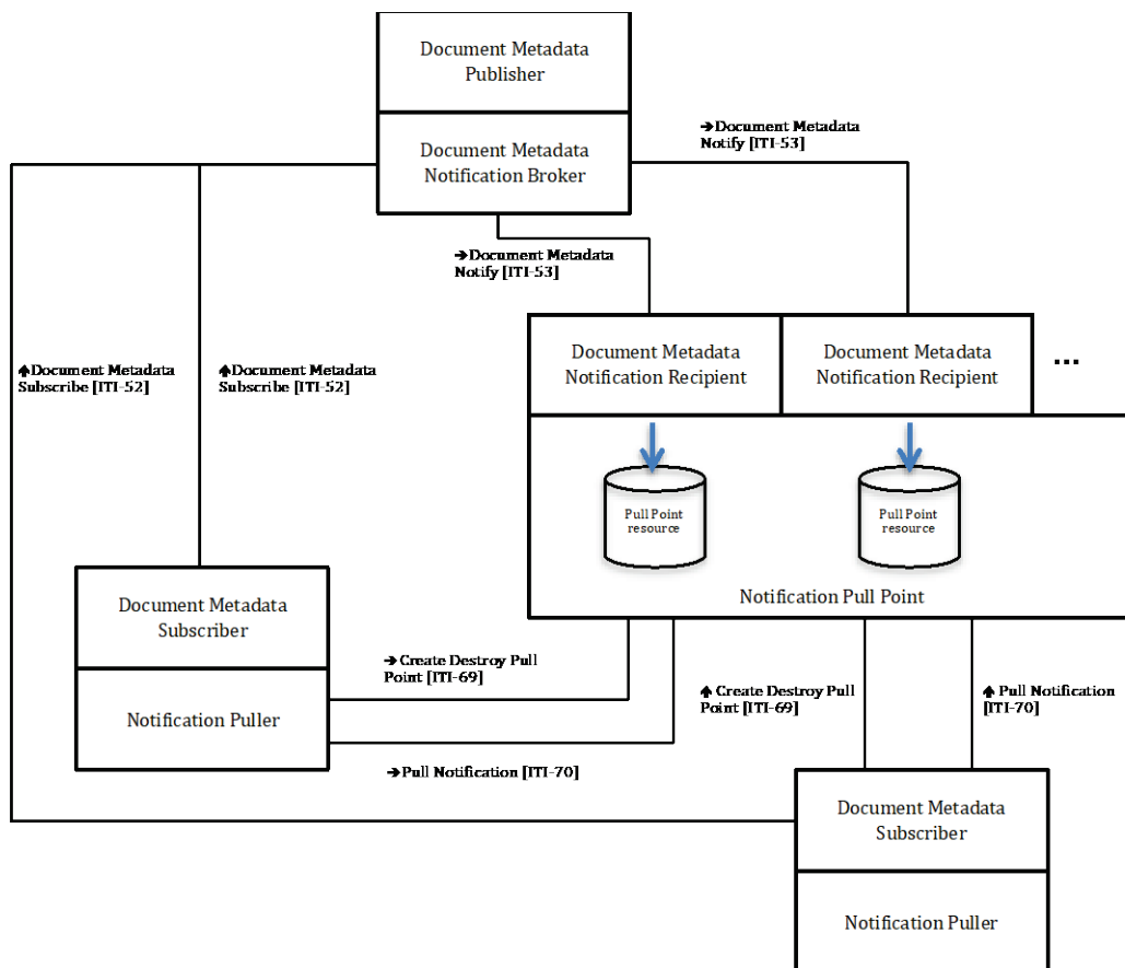
1045 Figure 3.69.4.1-1: Pull-style Notification Framework
