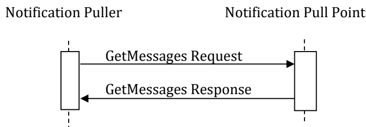
1225 Figure 3.70.4-1: Interaction Diagram
