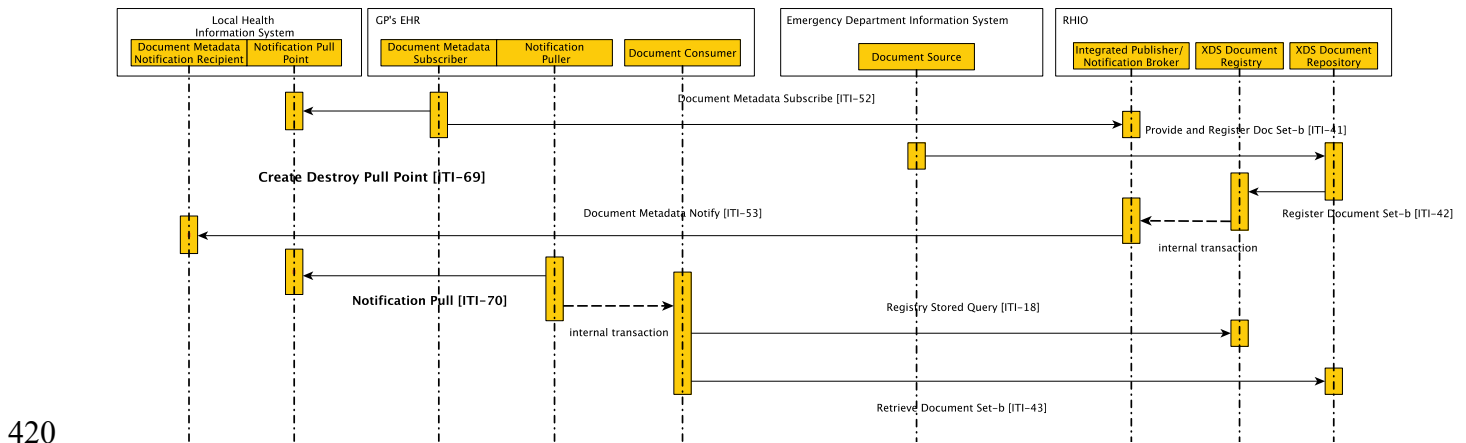
Figure 26.4.2.7.2-1: Sequence Diagram for GP’s EHR notification
