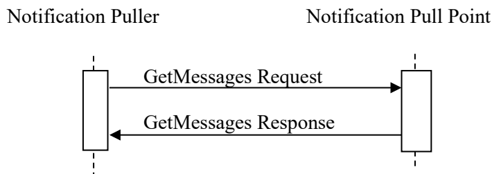
1885 Figure 3.70.4-1: Interaction Diagram
