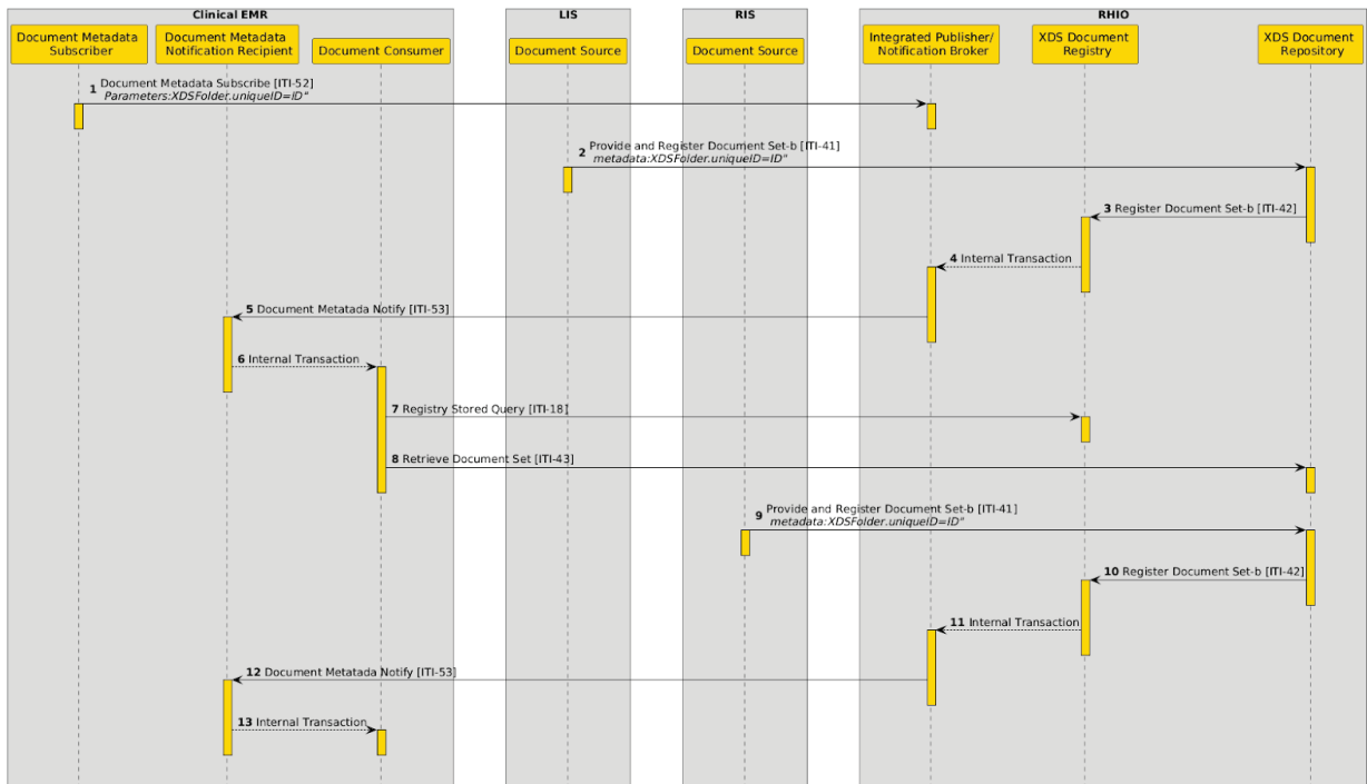
570 Figure 26.4.2.6.2-1: Interaction Diagram for Folder subscription Use Case
