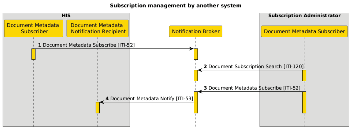
Figure 26.4.2.10.2-1: Interaction Diagram for Subscription management by other system
