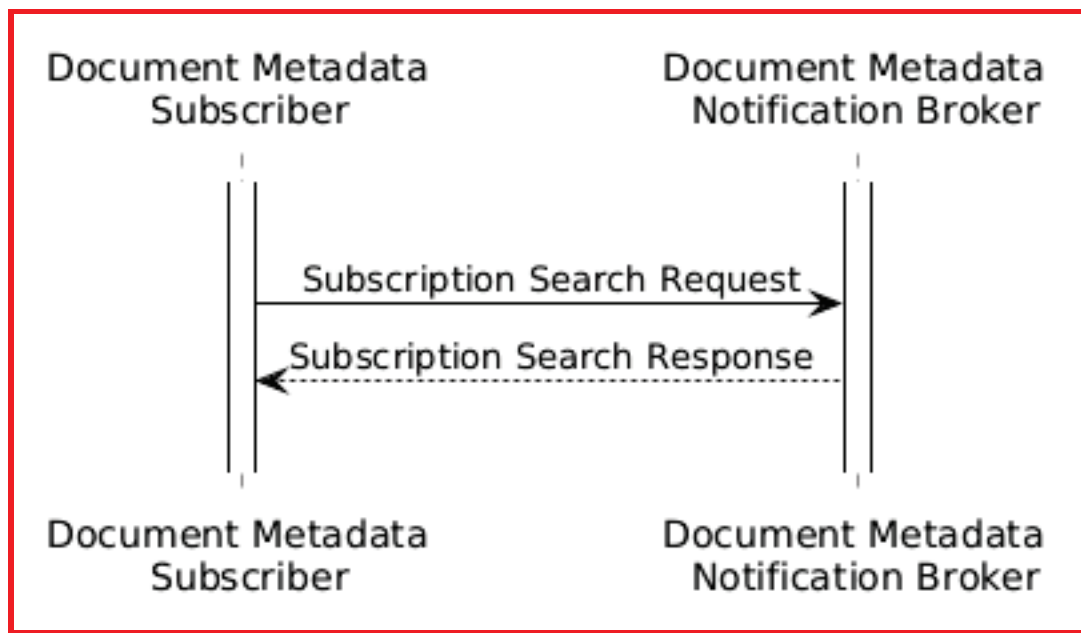
Figure 3.120.4-1: Document Subscription Search Sequence
