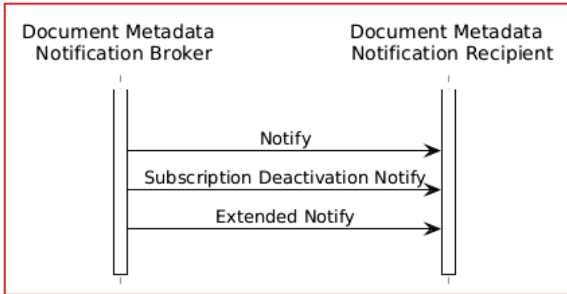
Figure 3.53.4-1: Document Metadata Notify Sequence
