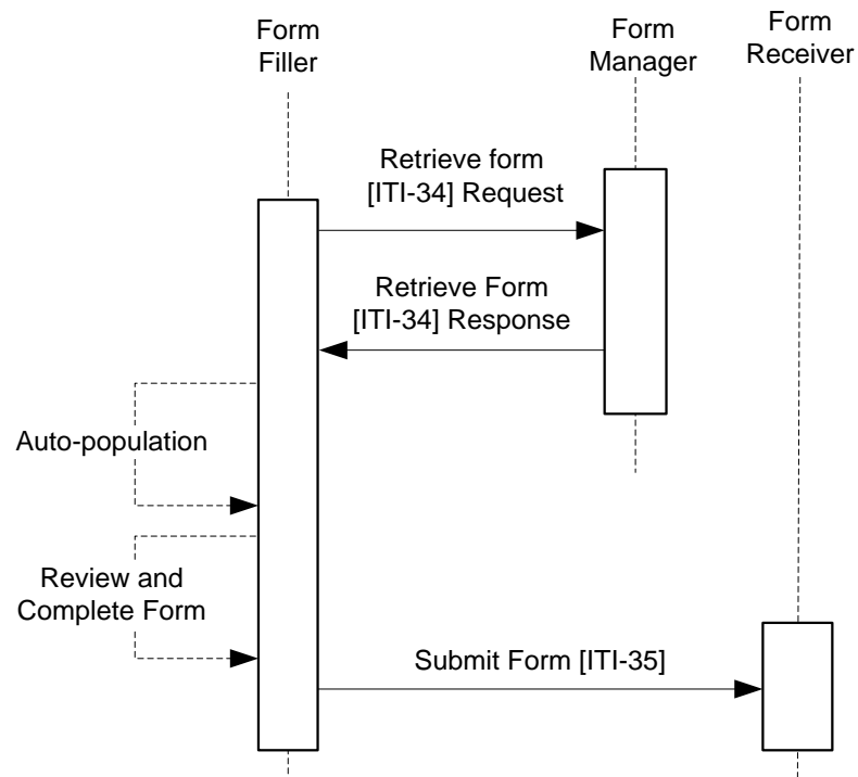
485 Figure X.4.2.2.2-1: Capture and Submit Pre-Authorization – Process Flow diagram
