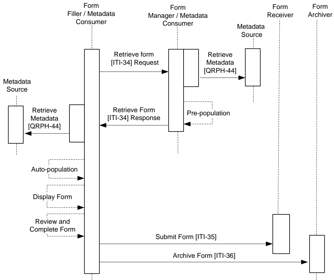
Figure X.4.2.3.2-1: SDC Profile Use Case with Extraction Specification - Process Flow diagram
