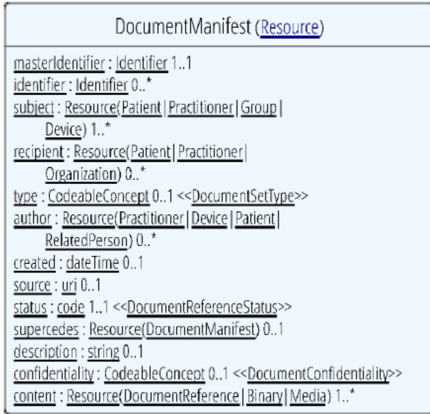
Figure 3.66.4.2.2-1: Document Manifest Resource definition (Diagram from HL7 FHIR, does not include IHE constraints)
