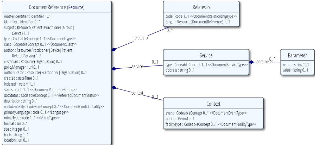
Figure 3.67.4.2.2-1: Document Reference Resource definition (From FHIR DSTU1 DocumentReference)
